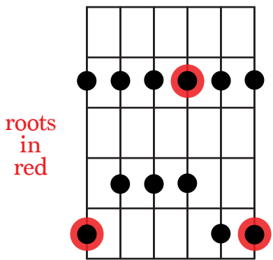
G shape Major Pentatonic Scale
