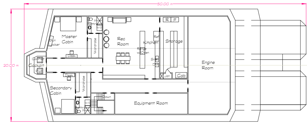
Living Level Plan View
